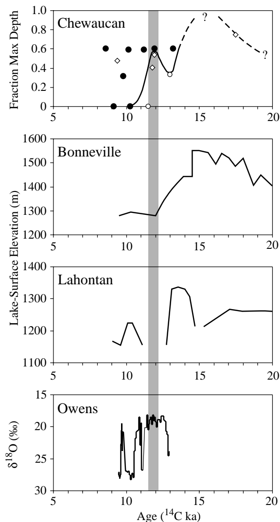
Figure 3 Lake-level curves and lake-size proxies of Great Basin pluvial lakes from 20 to 5 ^{14}\text{C} ka, arranged generally north (top panel) to south (bottom panel). The Lake Chewaucan curve is a composite record of lake-level data, normalised to the fraction of maximum lake depth, from the Chewaucan and Fort Rock basins (after Negrini, in press). Open diamonds denote material formed below lake-level in the Chewaucan basin. Open circles denote material formed below lake-level in the Fort Rock basin. Solid circles denote archaeological sites and other material formed above lake-level in the Fort Rock basin. The question mark obscuring the precise timing of the maximum highstand indicates the conjectural nature of its age, and dashed lines indicate poorly constrained portions of the curve. The stippled column identifies the approximate timing of the Chewaucan lake-level oscillation. The curves for lakes Bonneville and Lahontan are generalised from published data of Benson et al. (1995, 1997), Oviatt et al. (1992), Oviatt (1997), Adams and Wesnousky (1998), and references therein. The Owens Lake \delta^{18}\text{O} proxy data are from core OL84B using the age model of Benson (1999); \delta^{18}\text{O} minima (plotted as peaks) are proxies of wet oscillations in the basin
