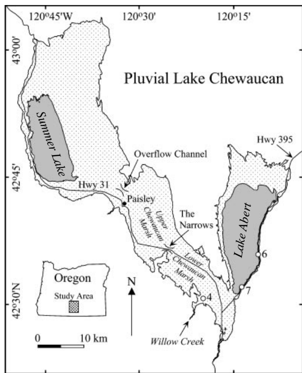
Figure 1 Location map for the Chewaucan basin. The extent of pluvial Lake Chewaucan at its maximum 1378 m highstand is shown as light stipple, and the modern remnants Summer Lake and Lake Abert are shown as darker stipple. Stratigraphical section locations are marked with numbered circles
