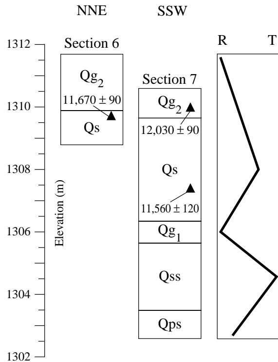
Figure 2 Measured stratigraphical sections 6 and 7 (see Fig. 1 for locations), with a schematic curve of regressive (R) and transgressive (T) lake cycles. Labelled stratigraphical units are described in the text. Black triangles mark the location of radiocarbon-dated gastropods. Ages are in ^{14}\text{C} yr BP
