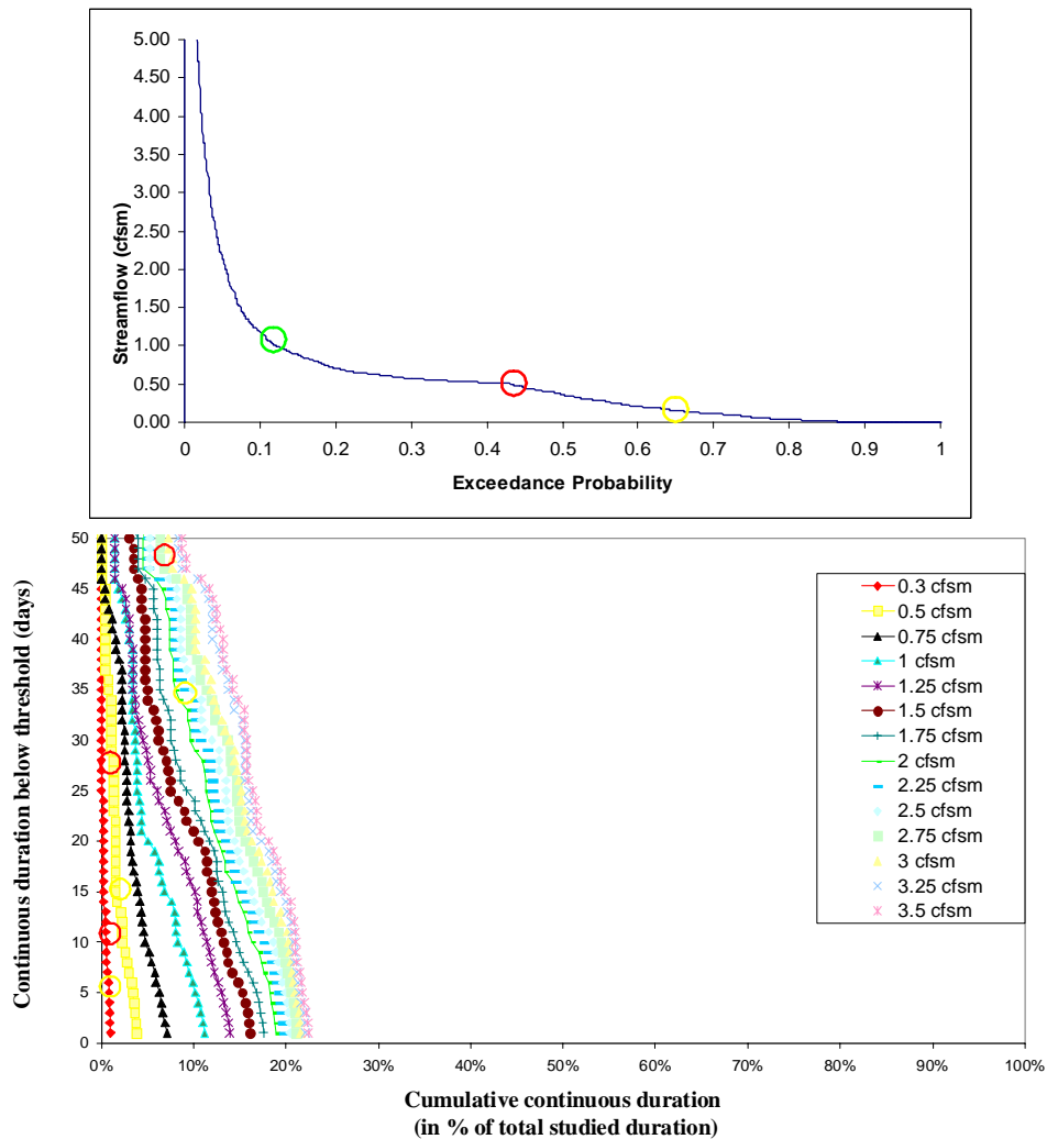
Figure 12: FDC and UCUT curves for overwintering bioperiod (Nov. 15 – Feb. 28).
