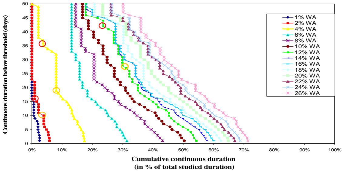
Figure 4: HDC and UCUT curves for Reach 2 R&G bioperiod based on Atlantic salmon habitat.
