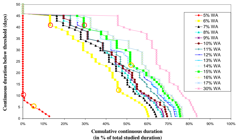
Figure 11: HDC and UCUT curves for Reach 5 Atlantic salmon spawning.
