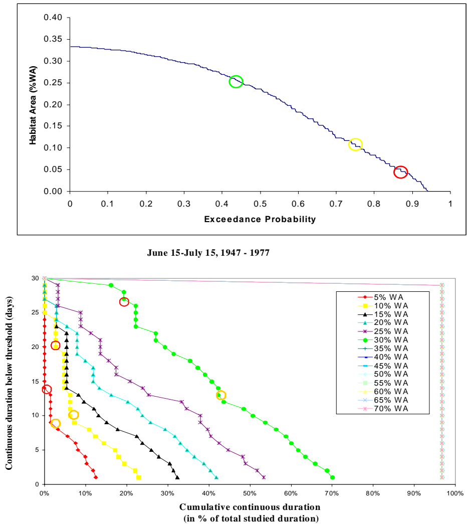
Figure 16: HDC and UCUT curves for Reach 2 GRAF spawning.
