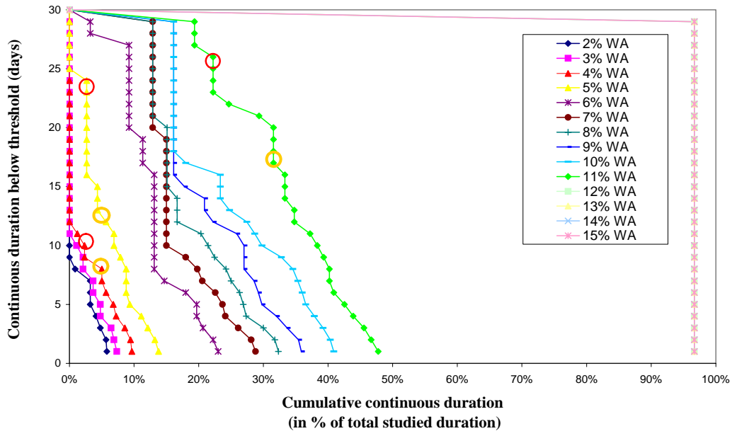
Figure 7: HDC and UCUT curves for Reach 5 GRAF spawning.
