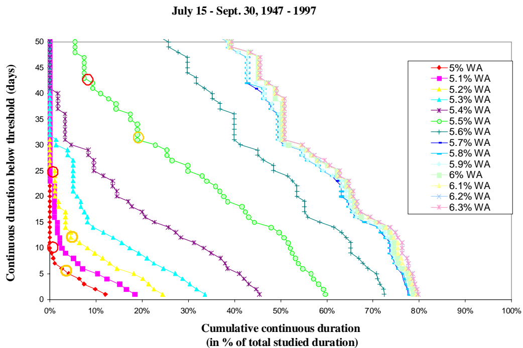
Figure 7: HDC and UCUT curves for Reach 5 R&G bioperiod.
